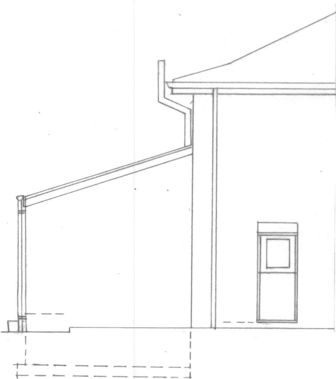
SOUTH ELEVATION
